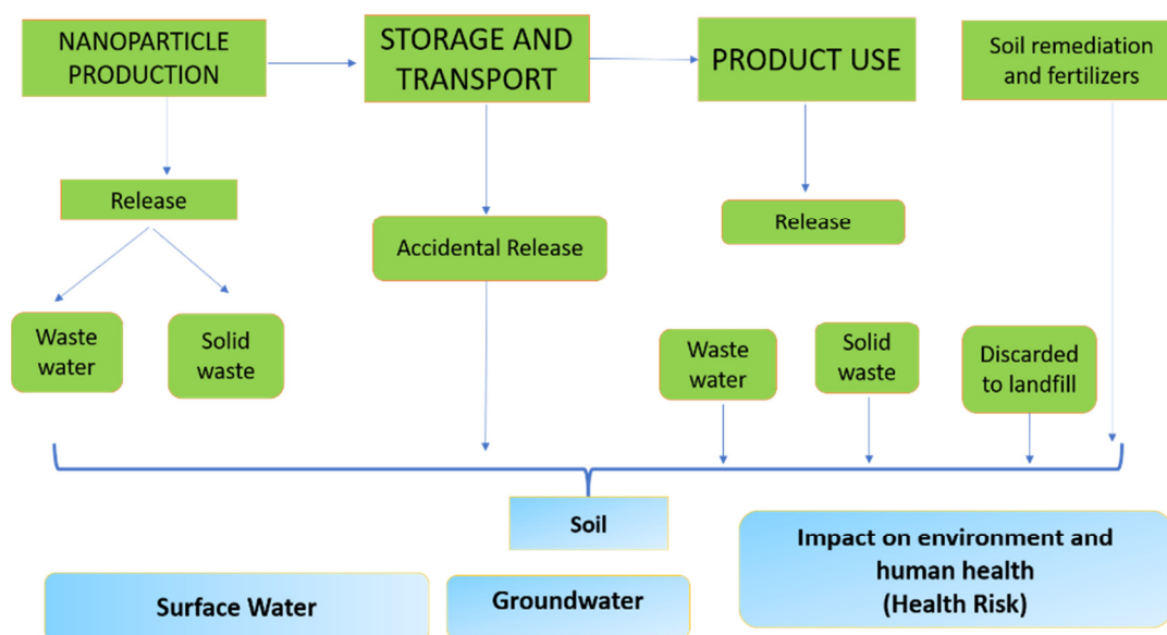
Fig 1. Sources of nanoparticles in different environmental media
