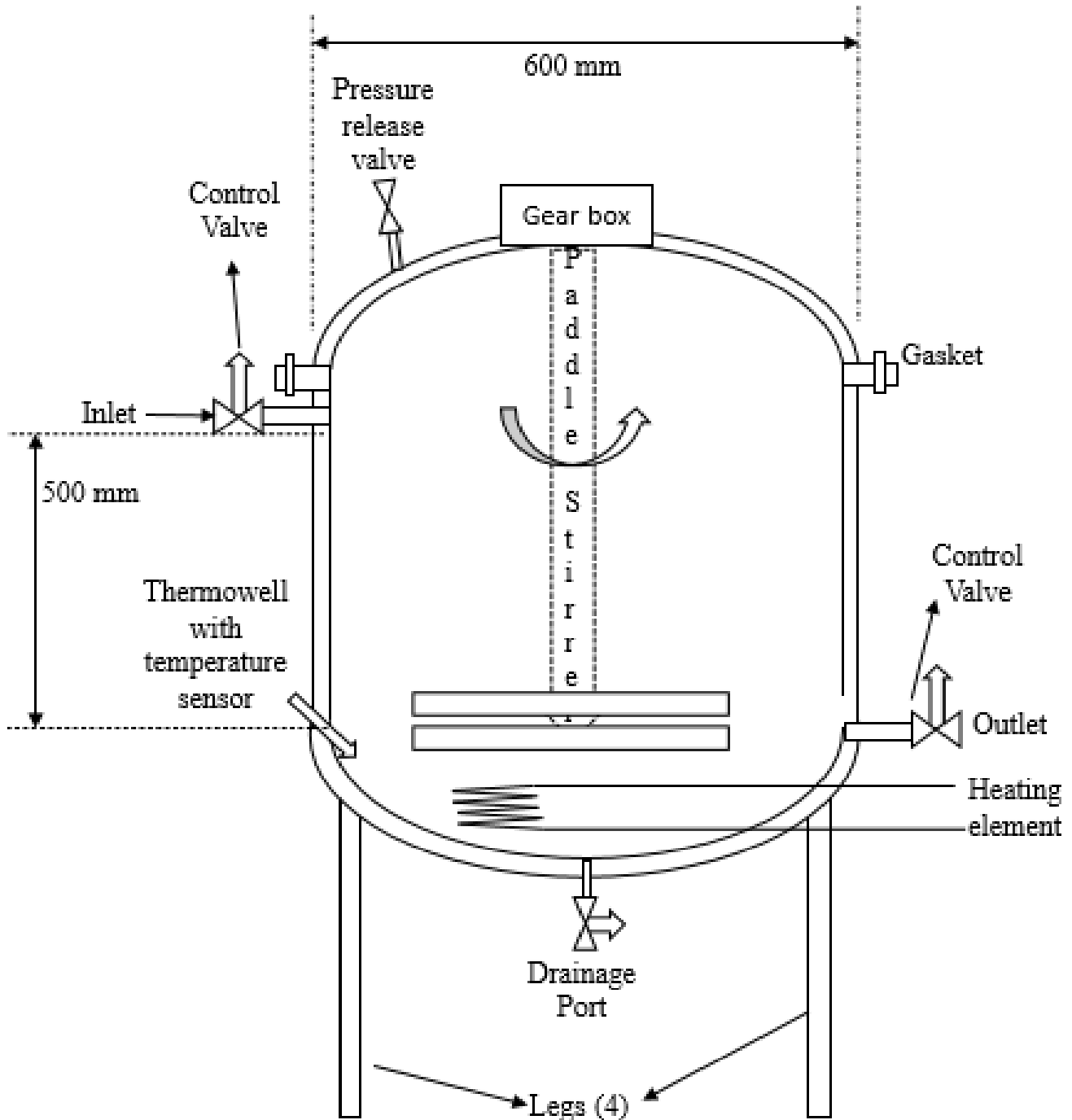
Fig. 1: Schematic of Medium Temperature Thermal Bath
