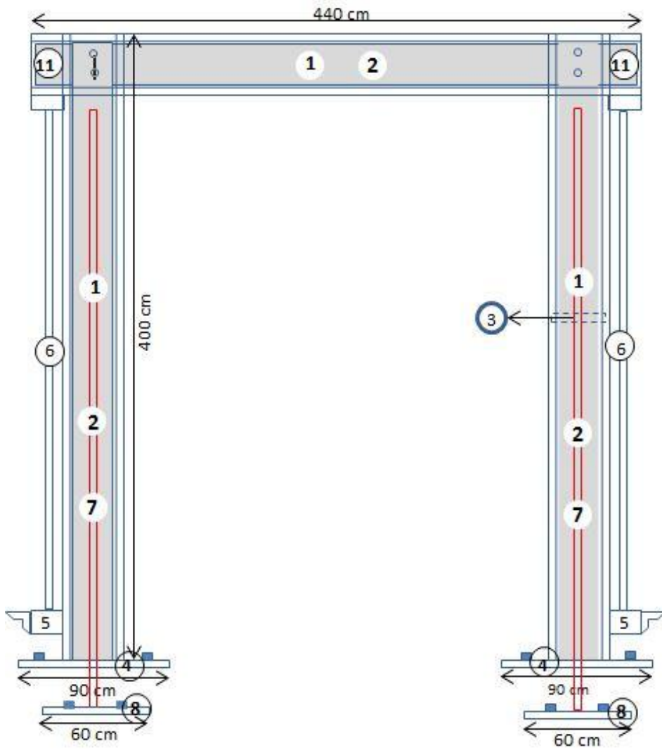
Figure 1 Section of the Loading Frame
