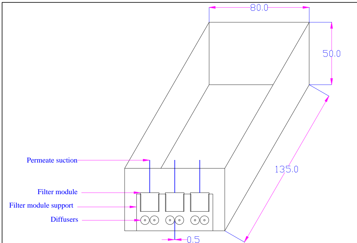
Fig 3: Filtration unit
