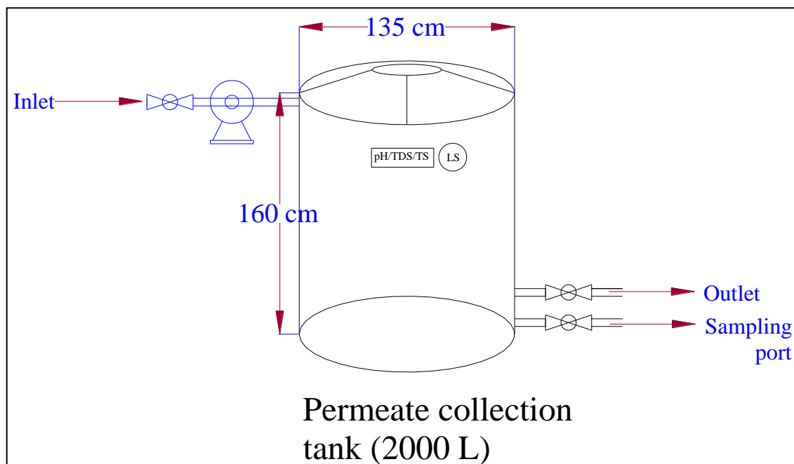
Fig 5: Permeate tank
