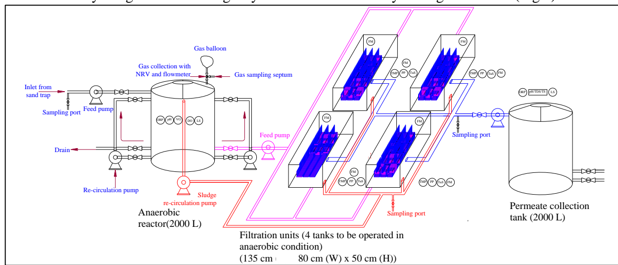
Fig 1: Indicative layout of the AnMBR system
