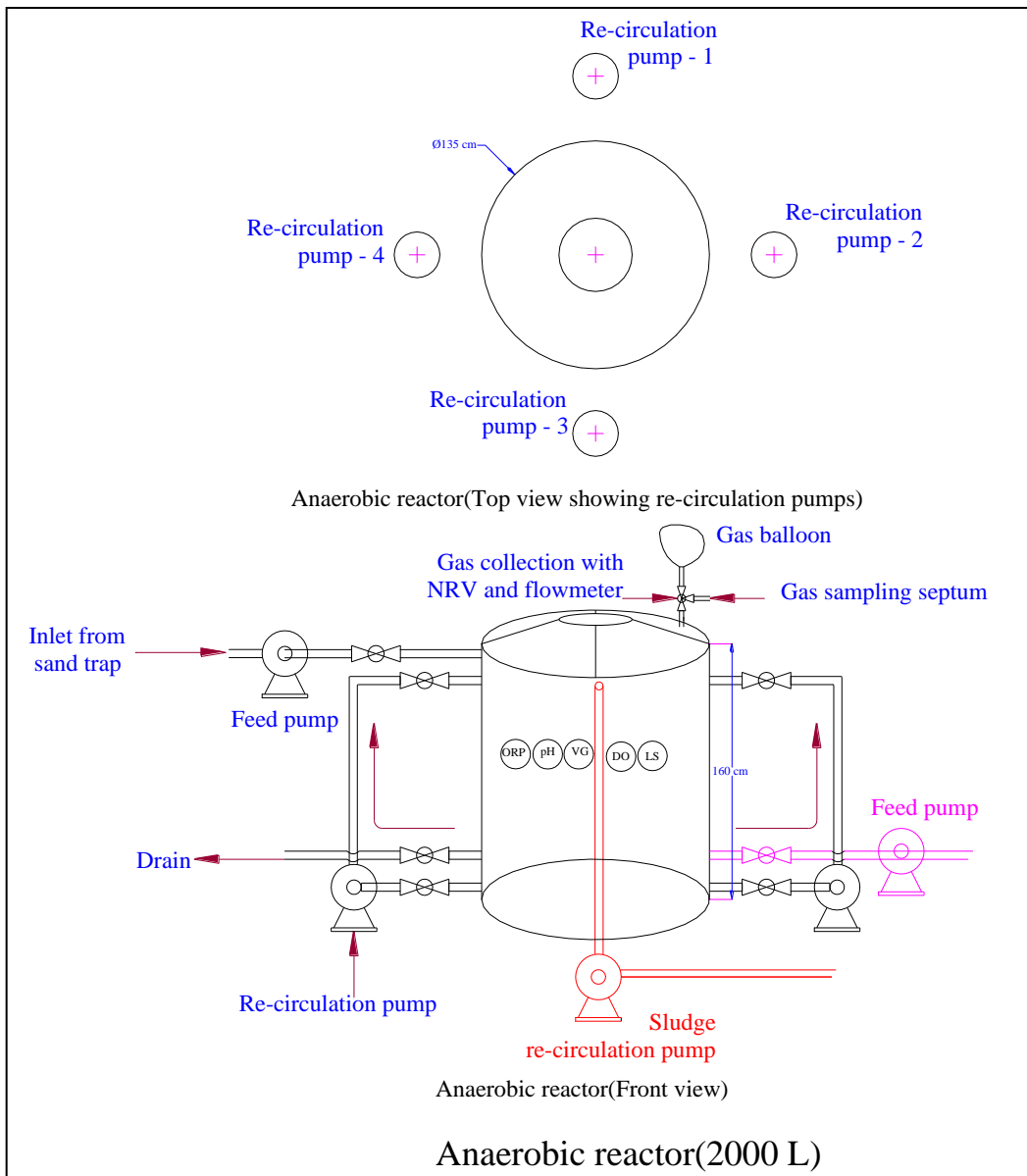
Fig 2: Anaerobic CSTR
