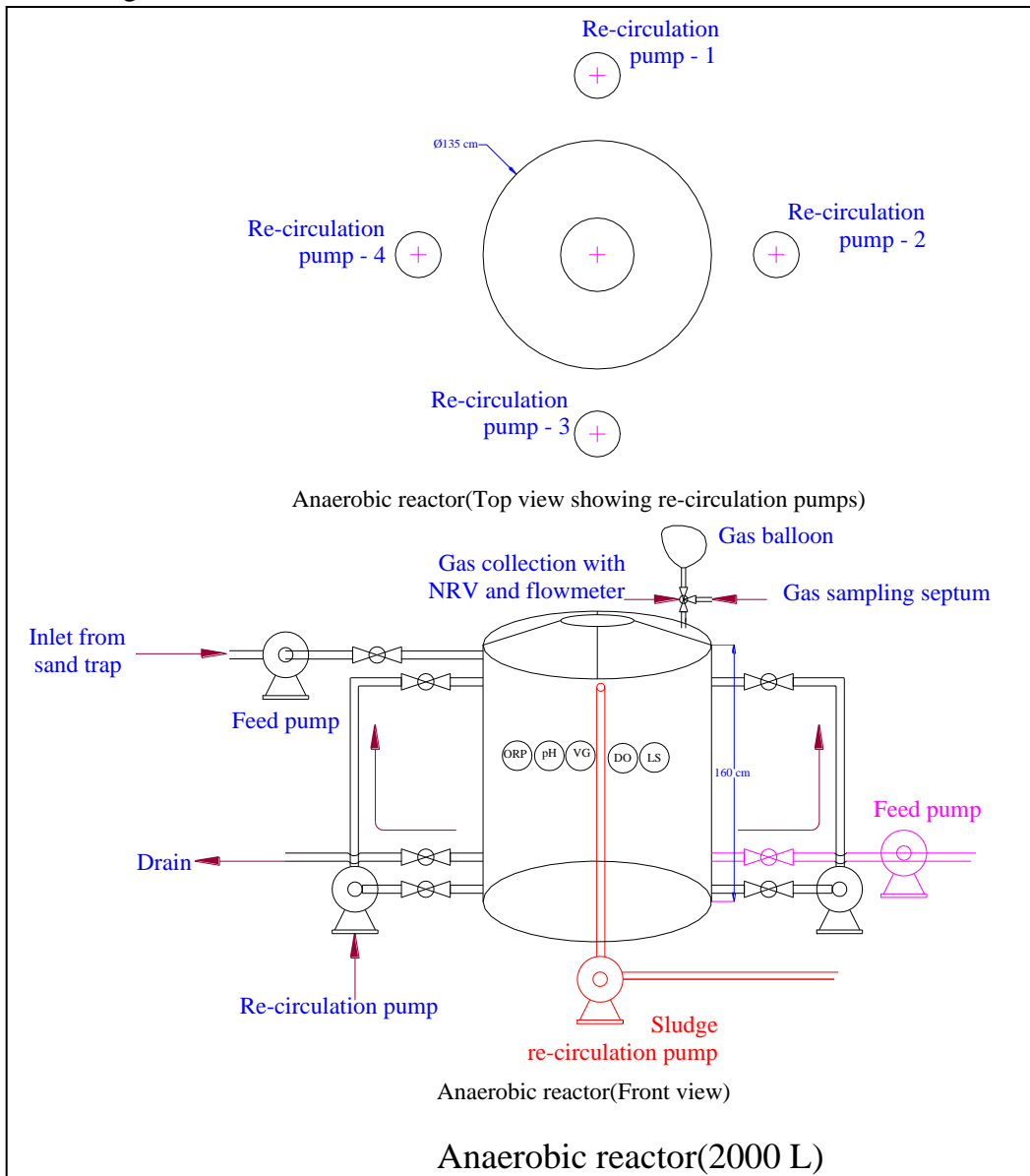
Fig 2 shows the details of the anaerobic CSTR.
