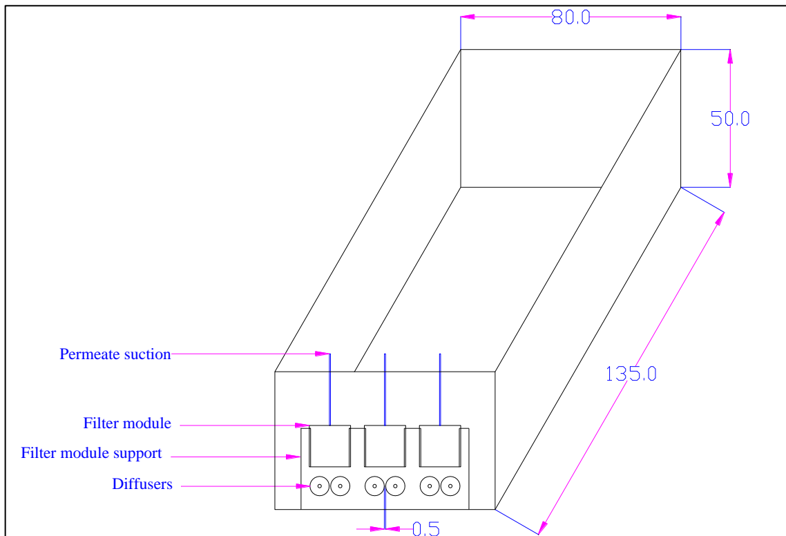
Fig 3: Filtration unit
