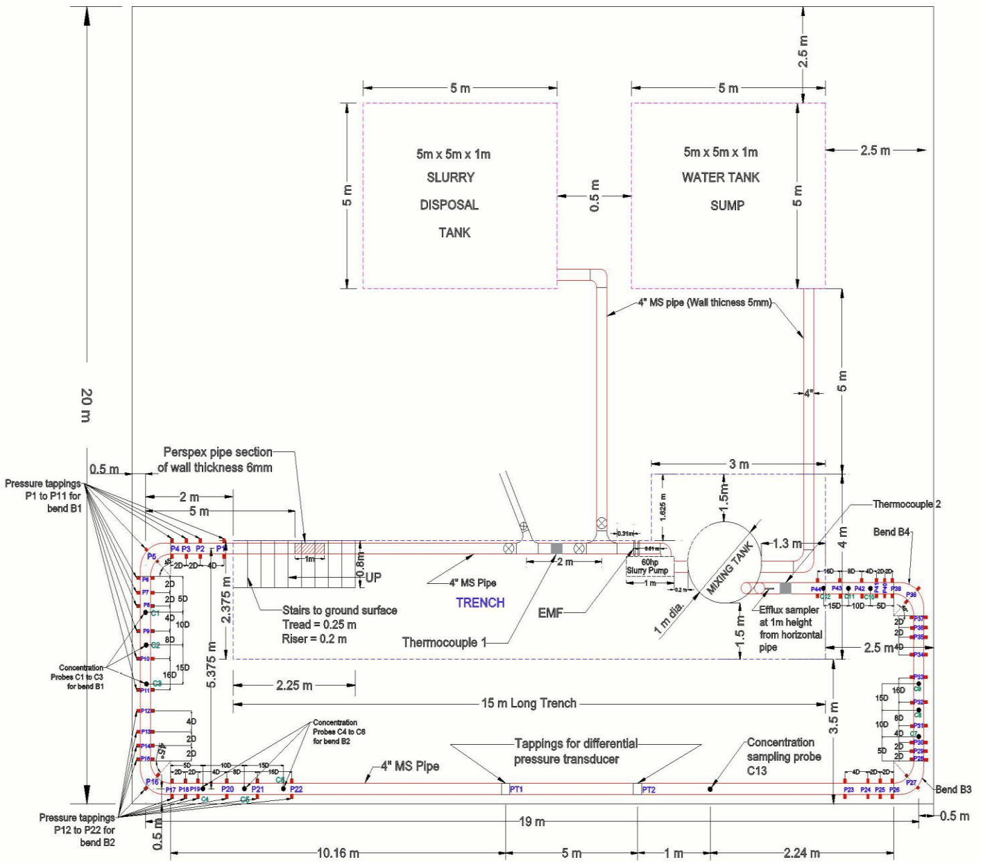
2D PLAN OF PIPE LOOP SETUP
