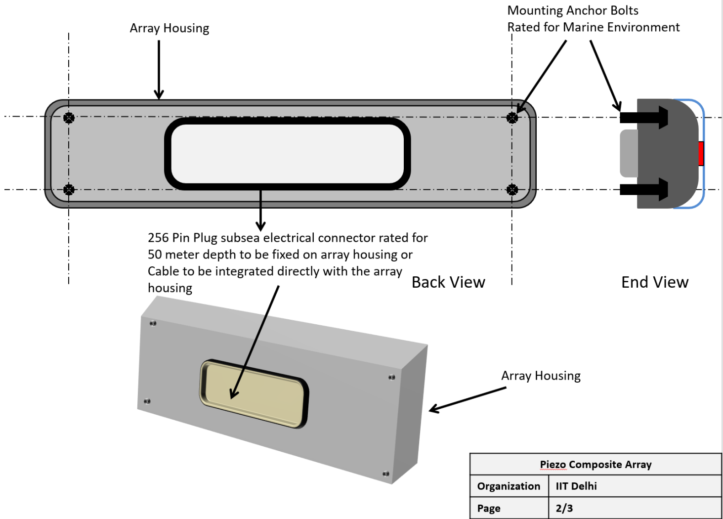
Figure 2: Back and end views of the array housing.
