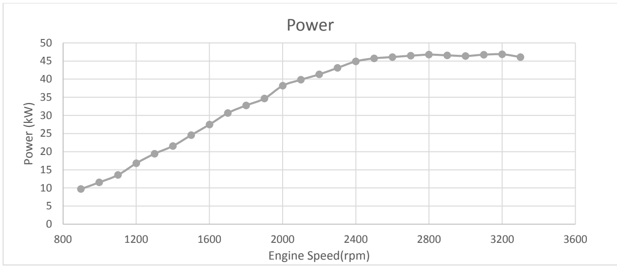
Fig. 2 Variation of power with respect to engine speed
