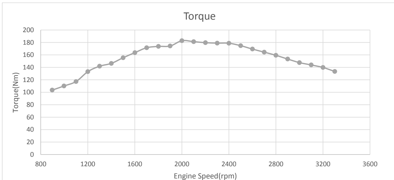
Fig. 1 Variation of torque with respect to engine speed
