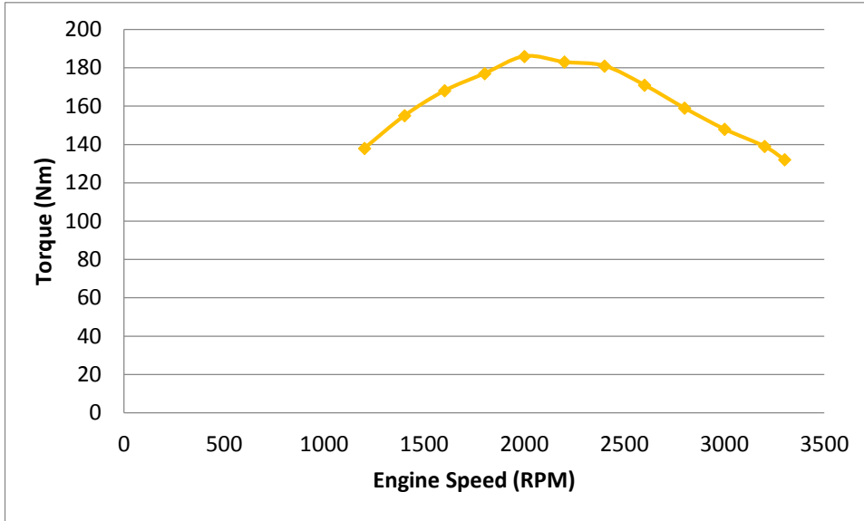
Figure 1: Engine speed vs Torque characteristic of engine
