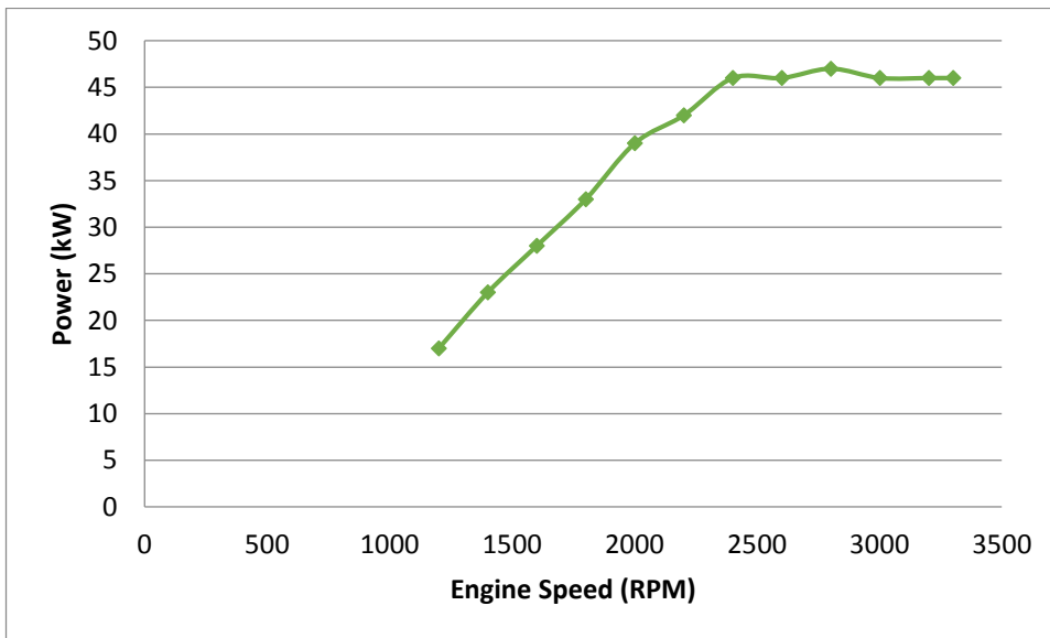
Figure 2: Engine speed vs Power characteristics of engine
