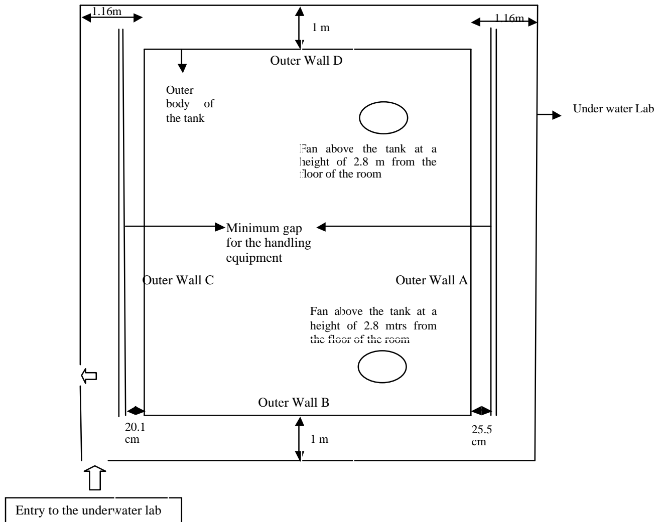
Fig 5. Layout of the underwater lab
