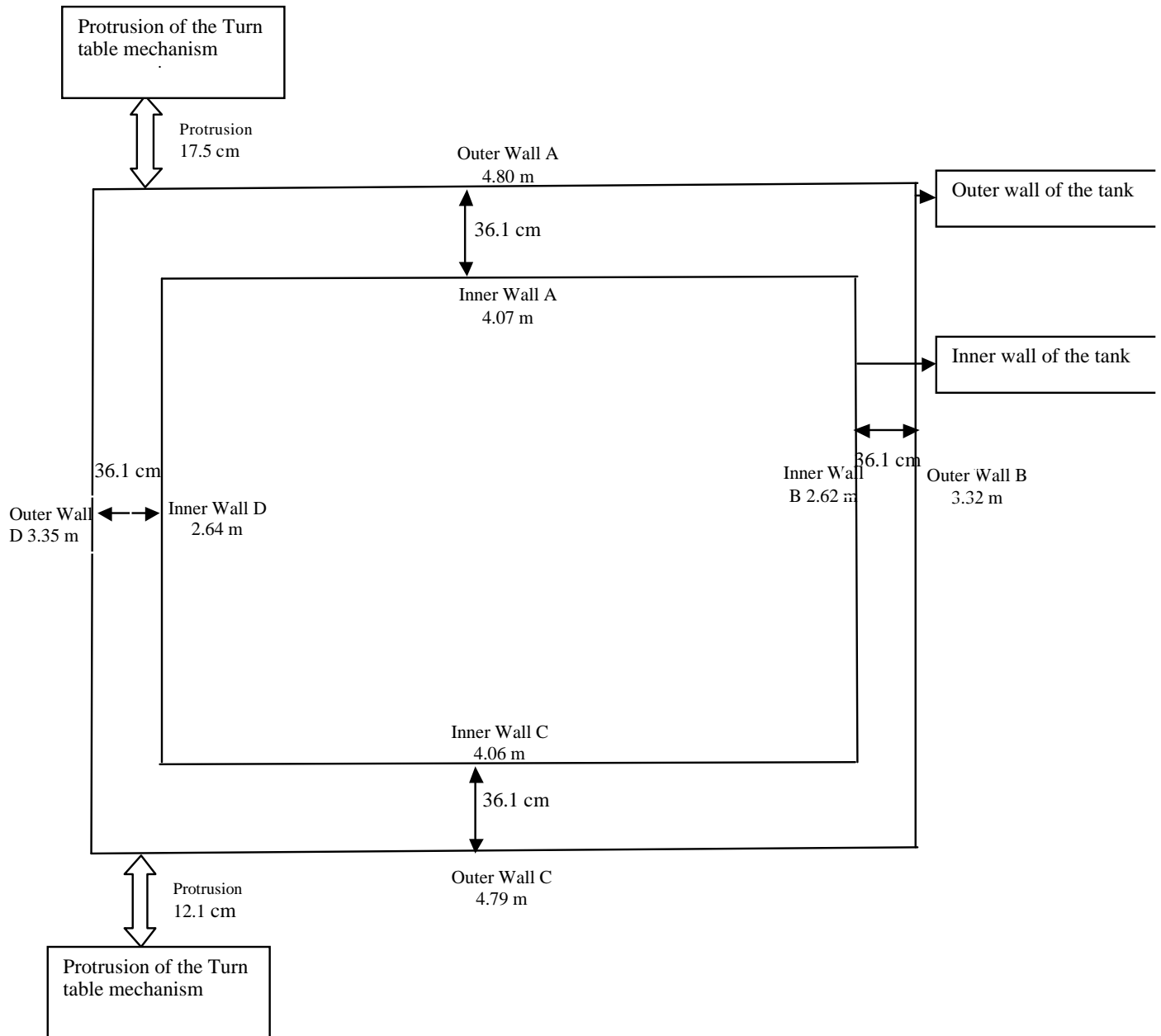
Fig 4. Top View of the tank
