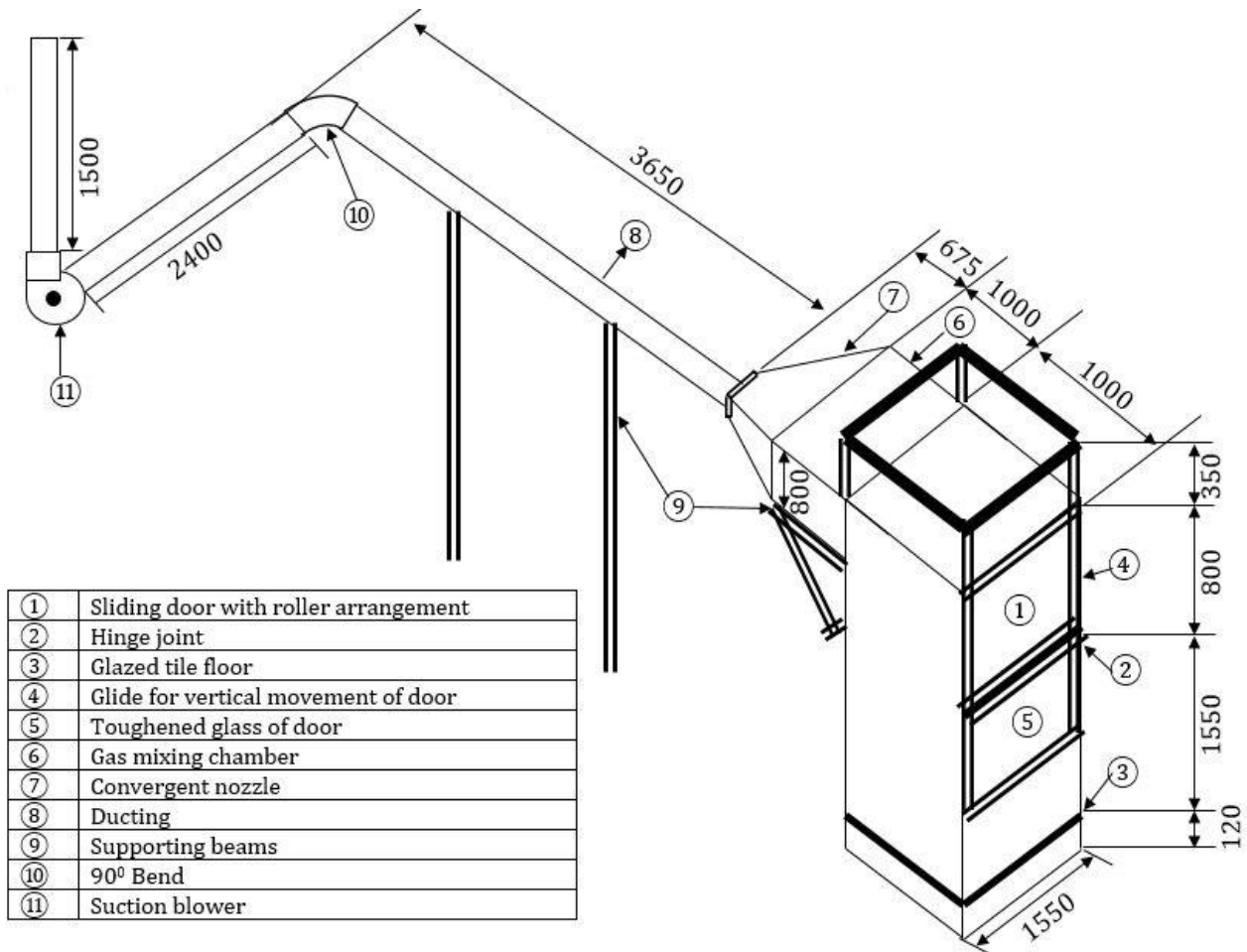
Layout of Fume Hood and duct with suction blower controlled by VFD
