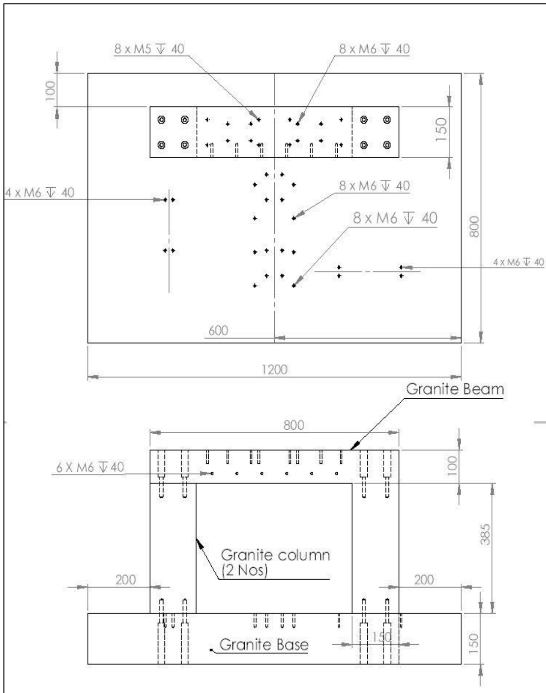
Figure 1: Dimensions of Granite Assembly
