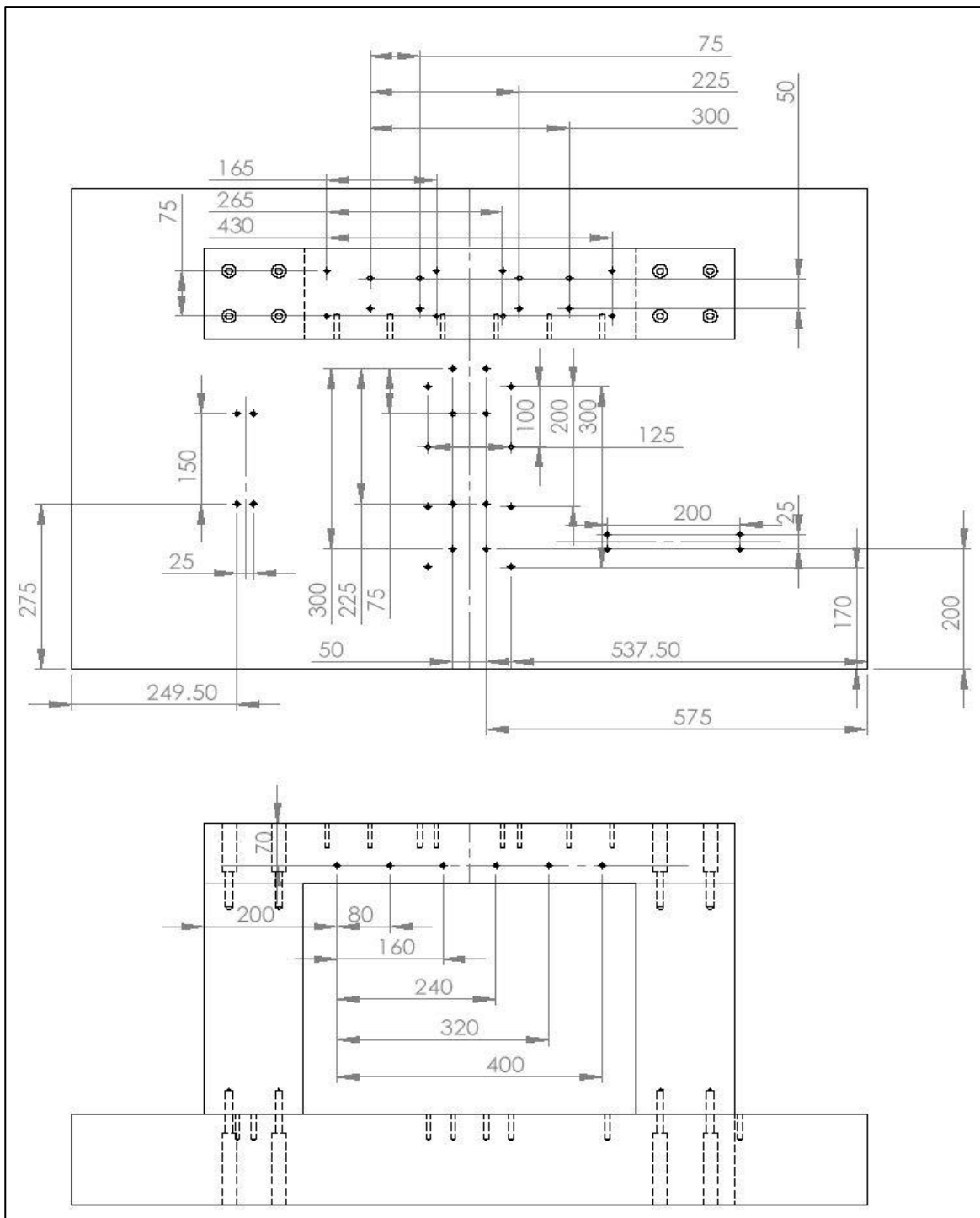
Figure 2: Dimensions of tap holes
