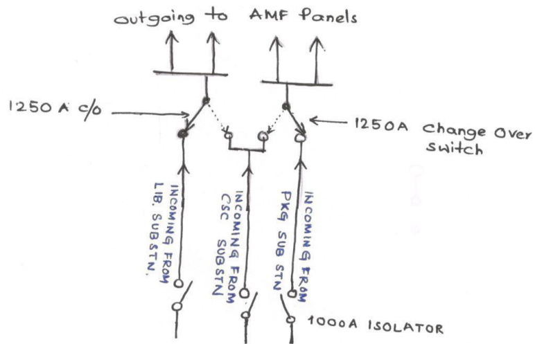
SCHEMATIC DIAGRAM
