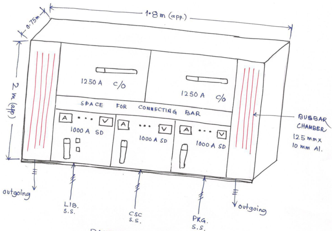
PANEL DIAGRAM (NOT TO SCALE)
