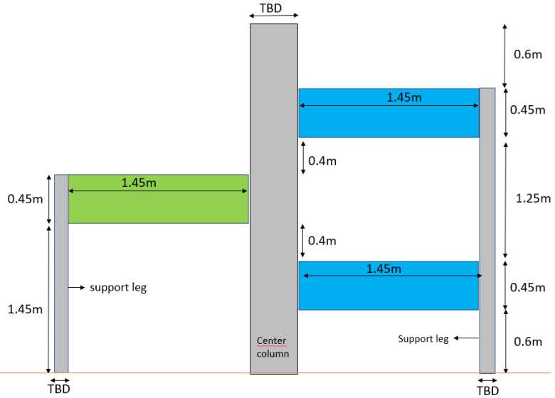
(Front/Side View)
