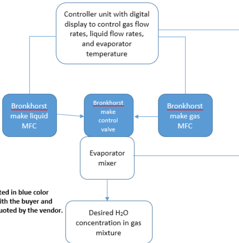
Figure 1. Required setup
