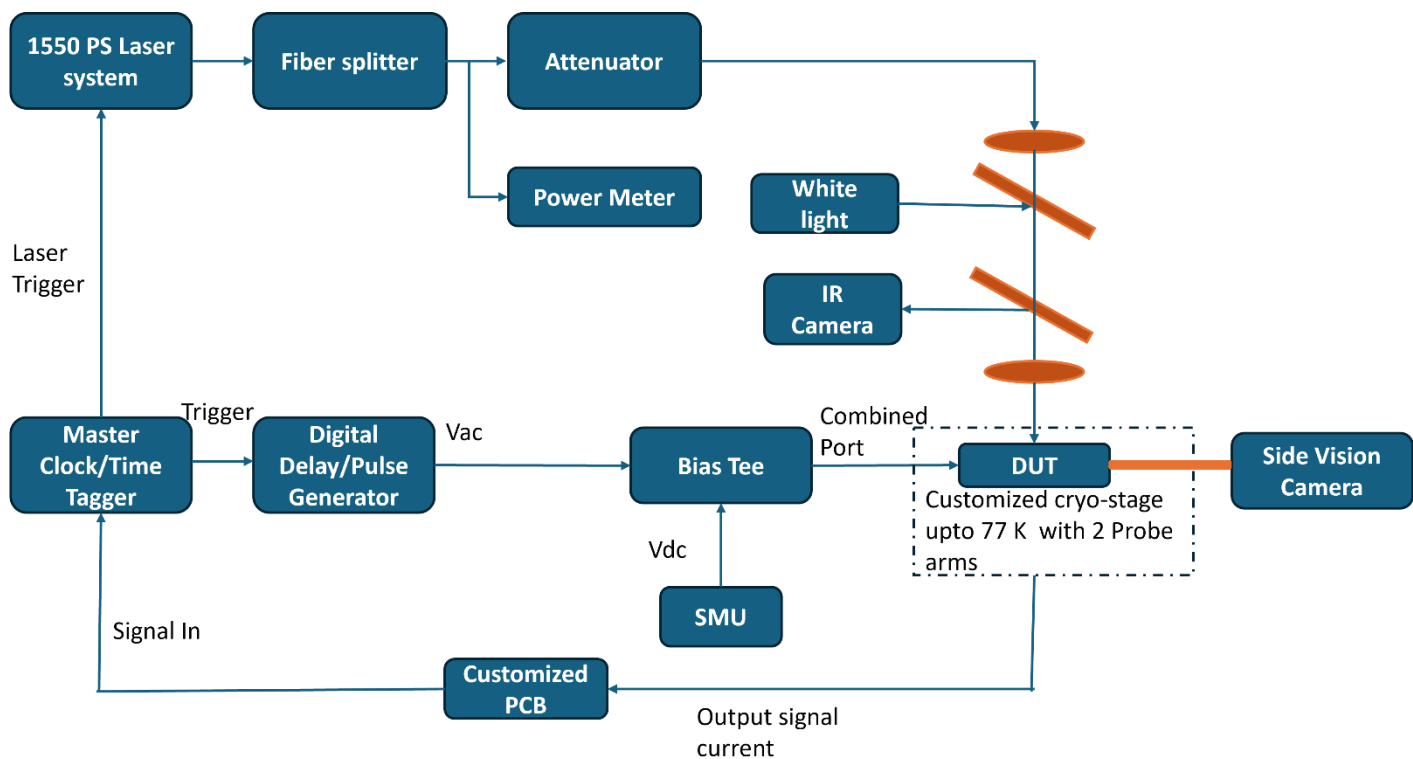
Figure 1. Schematic for SPAD characterization.
